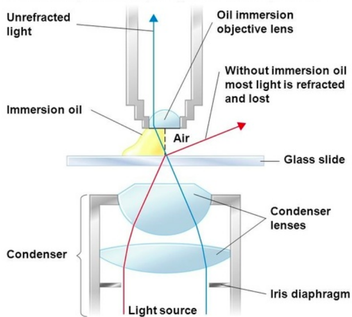
Figure 3. Comparison between the effects of immersion oil and air on the passage of light rays from a specimen to the front lens of the oil immersion objective.
