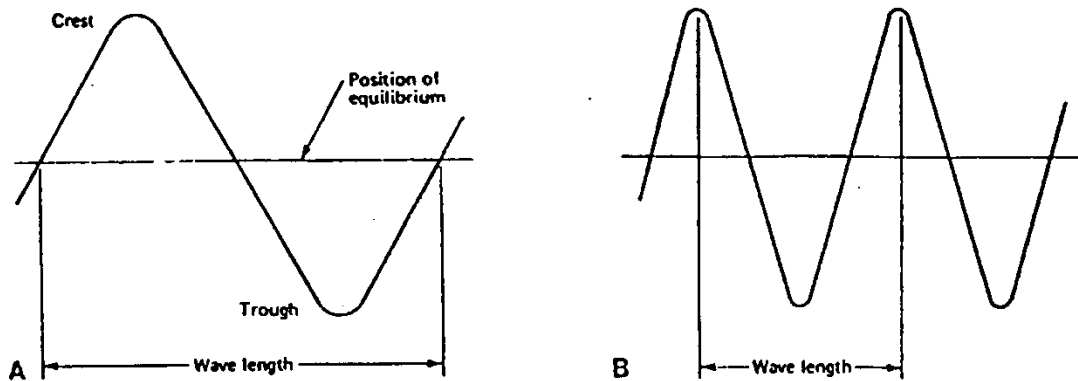
FIG. 1 Properties of light waves. A. The anatomy of a wavelength. Note the position of equilibrium. B. A representation of frequency.
