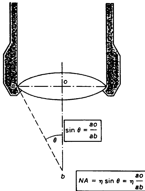
Figure 2 A diagrammatic representation of numerical aperture. (NA).
